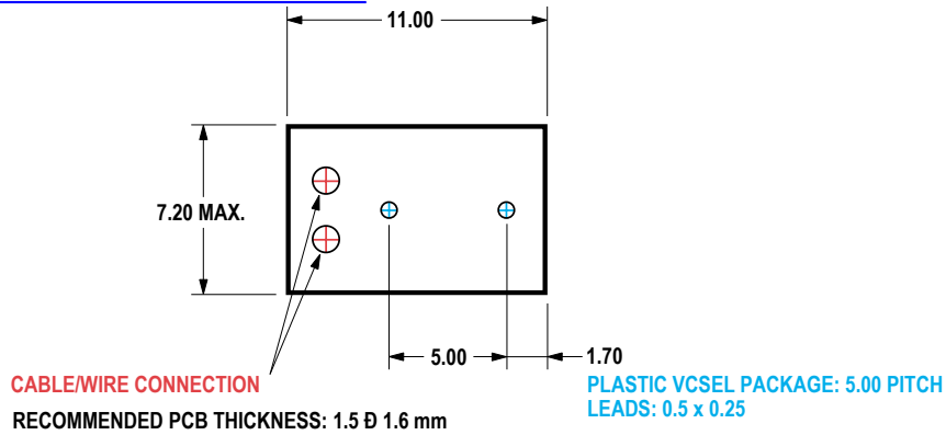
Figure 32. Suggested ADNV-6330 PCB mounting guide.
