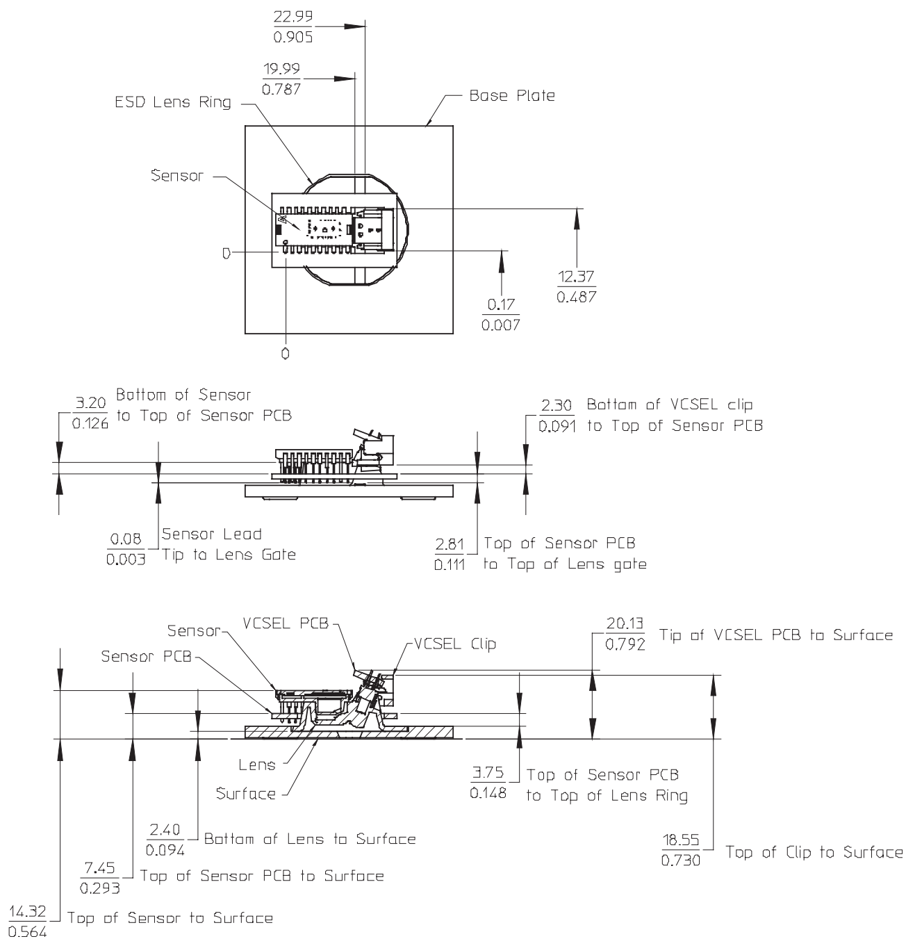
Figure 1. Assembly drawing of ADNB-6011 (top, front and cross-sectional view)
