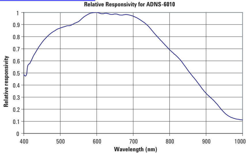
Figure 15. Relative Responsivity
