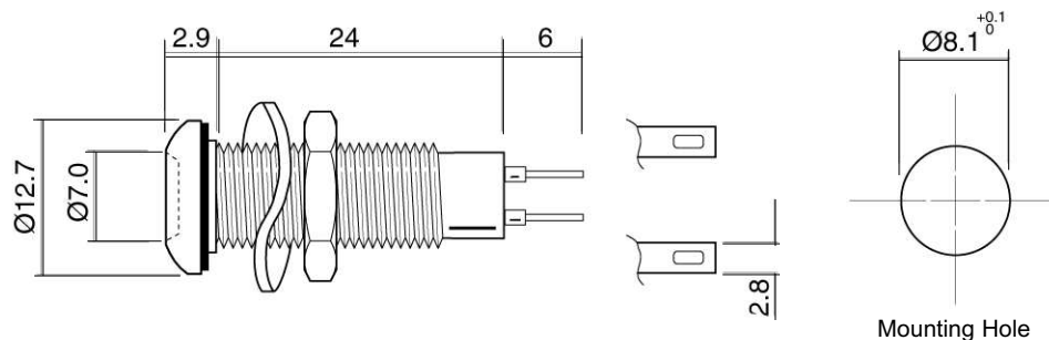
Mounting Hole
