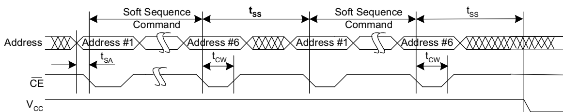
Figure 13. Soft Sequence Processing [25, 26]
