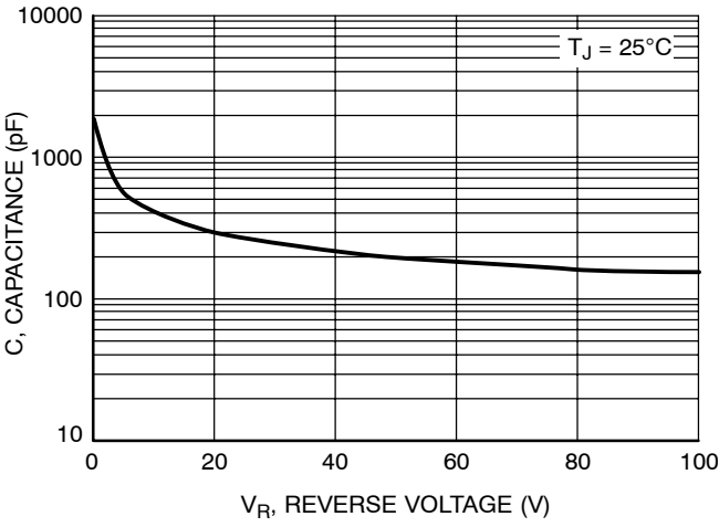
Figure 8. Capacitance
