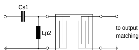
Fig. 4 series C – shunt L matching
