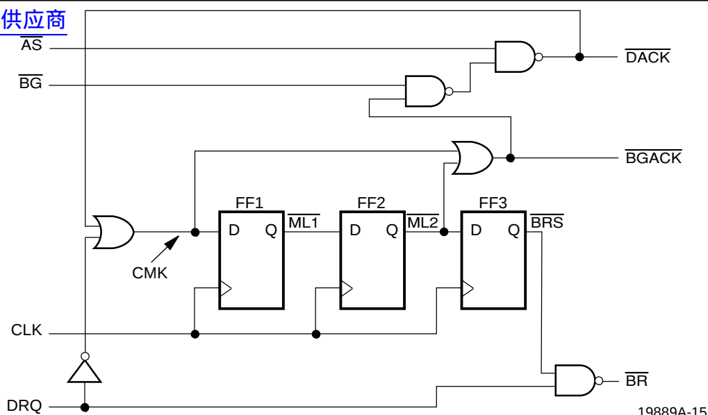
Figure 14. Bus Master Exchange Circuit
