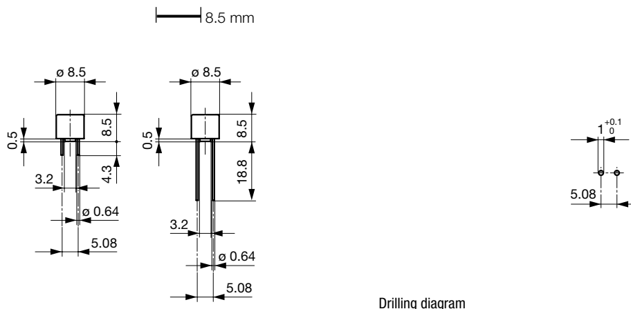
Drilling diagram
