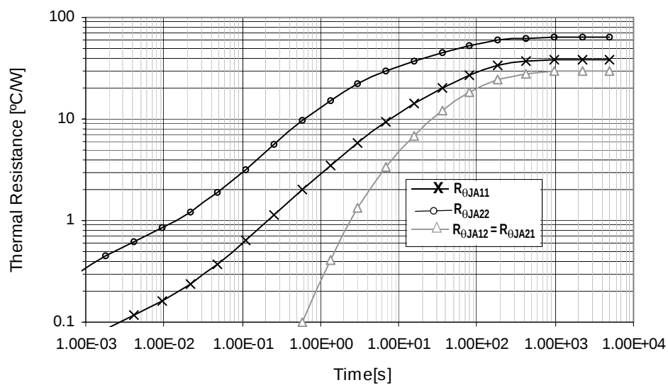
Figure 4. Transient Thermal Resistance R_{\theta JA} (1 W Step Response) Device on Thermal Test Board Area A = 600 (mm²)
