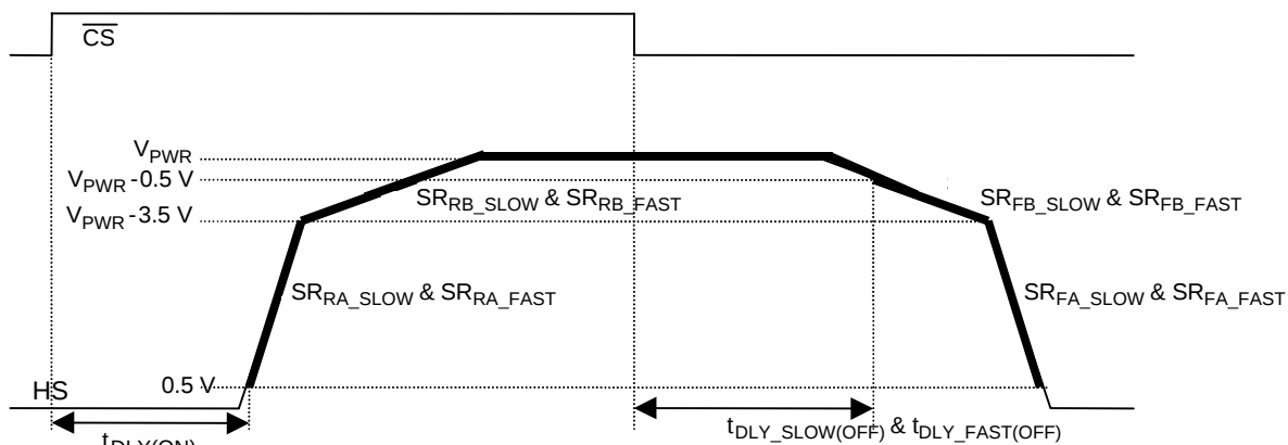
Figure 4. Output Slew Rate and Time Delays
