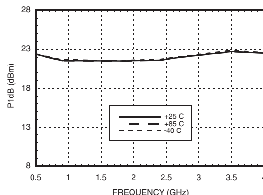
Output P1dB vs. Temperature
