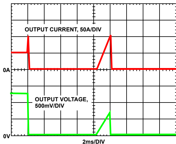
FIGURE 14. OVERCURRENT BEHAVIOR IN HICCUP MODE F_{\text{SW}} = 500\text{kHz}
