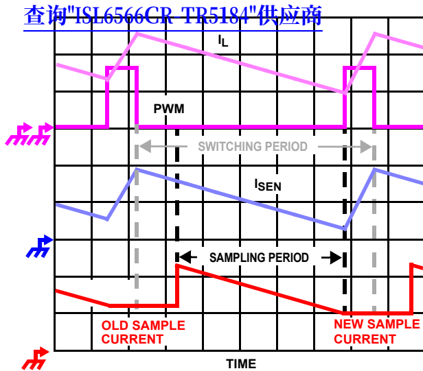
FIGURE 4. SAMPLE AND HOLD TIMING
