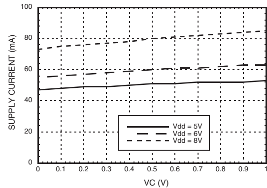
Supply Current vs. Vdd @ 22.5 Gbps [3]
