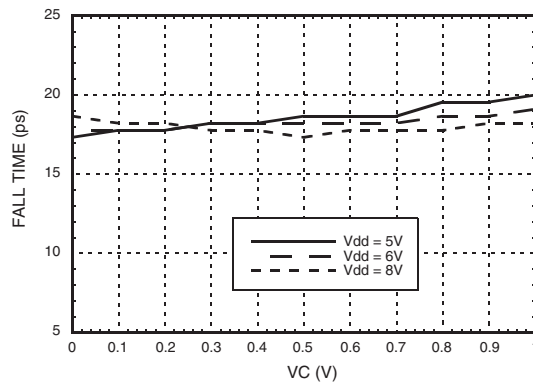
Fall Time vs. Vdd @ 22.5 Gbps [2]
