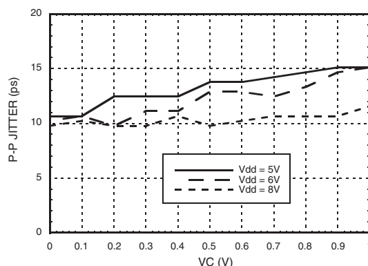
Peak-to-Peak Jitter vs. Vdd @ 22.5 Gbps [2]
