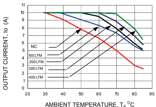
Figure 21. Derating Output Current versus Local Ambient Temperature and Airflow ( V_{in} = 12.0 \text{ Vdc} , V_o = 3.3 \text{ Vdc} ).
