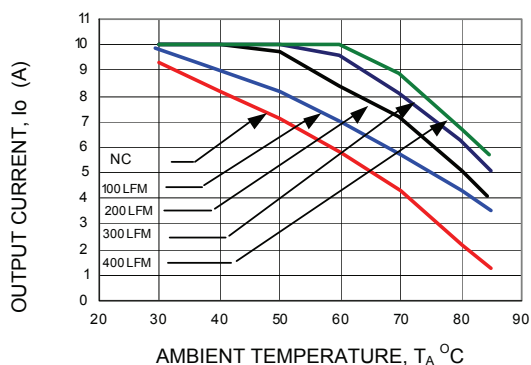
Figure 22. Derating Output Current versus Local Ambient Temperature and Airflow ( V_{in} = 12.0 \text{ Vdc} , V_o = 5.0 \text{ Vdc} ).
