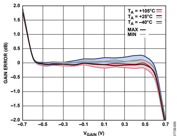
Figure 4. Gain Error vs. V_{\text{GAIN}} vs. Temperature
