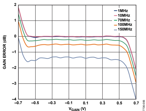
Figure 5. Gain Error vs. V_{\text{GAIN}} at Various Frequencies to VGAx
