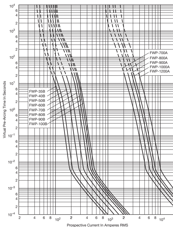
Time-Current Curve
