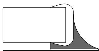
Good solder joint TNT0565-G-E
