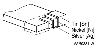
Figure 1 SMD NTC thermistors, structure of nickel barrier termination
