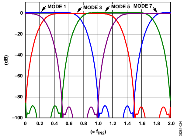
Figure 52. HB2, Odd Filter Modes
