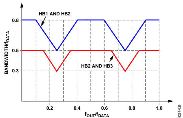
Figure 56. Signal Bandwidth vs. Center Frequency of the Output Signal, 4× Interpolation
