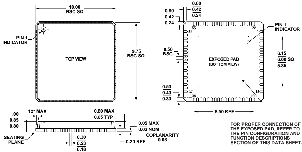
Figure 86. 72-Lead Lead Frame Chip Scale Package [LFCSQ_VQ] 10 mm × 10 mm Body, Very Thin Quad (CP-72-7)
