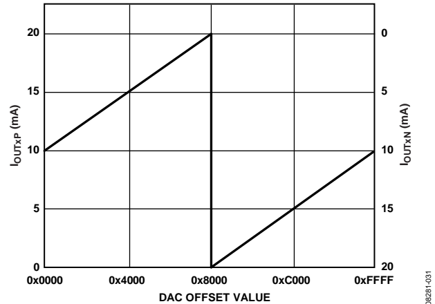
Figure 59. DAC Output Currents vs. DAC Offset Value
