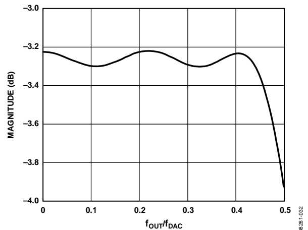
Figure 60. Sample Composite Responses of the \text{Sinc}^{-1} Filter with \text{Sin}(x)/x Roll-Off
