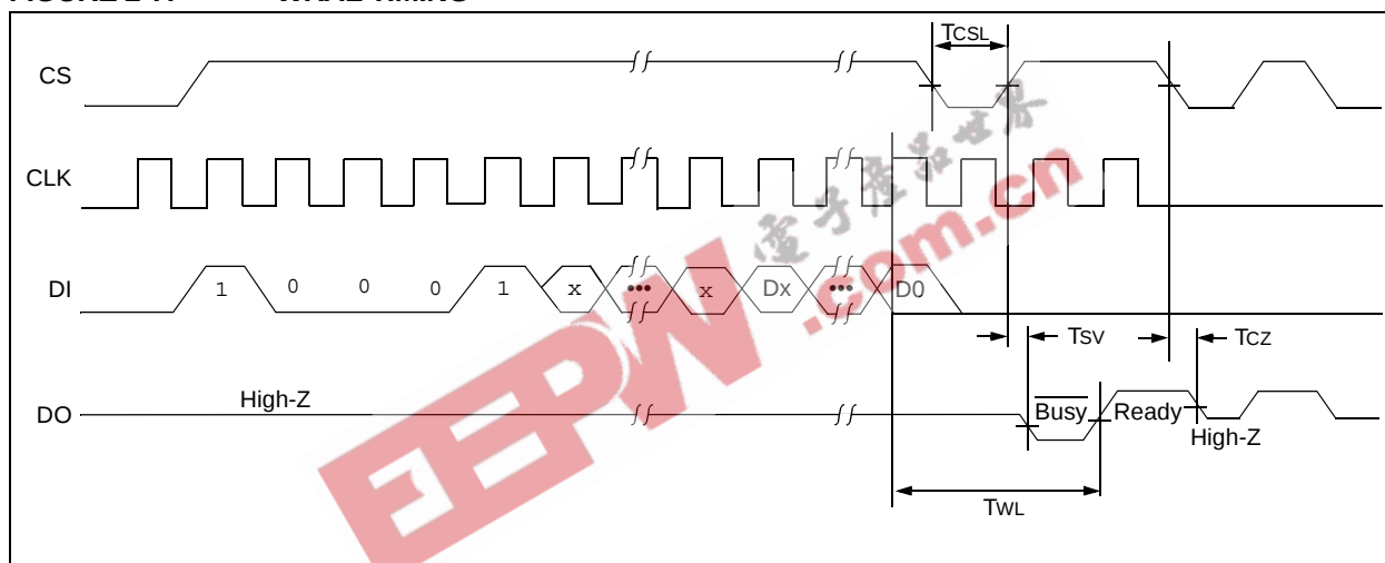
FIGURE 2-7: WRAL TIMING
