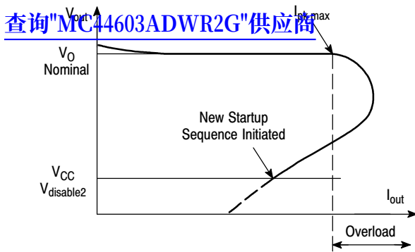
Figure 46. Foldback Characteristic
