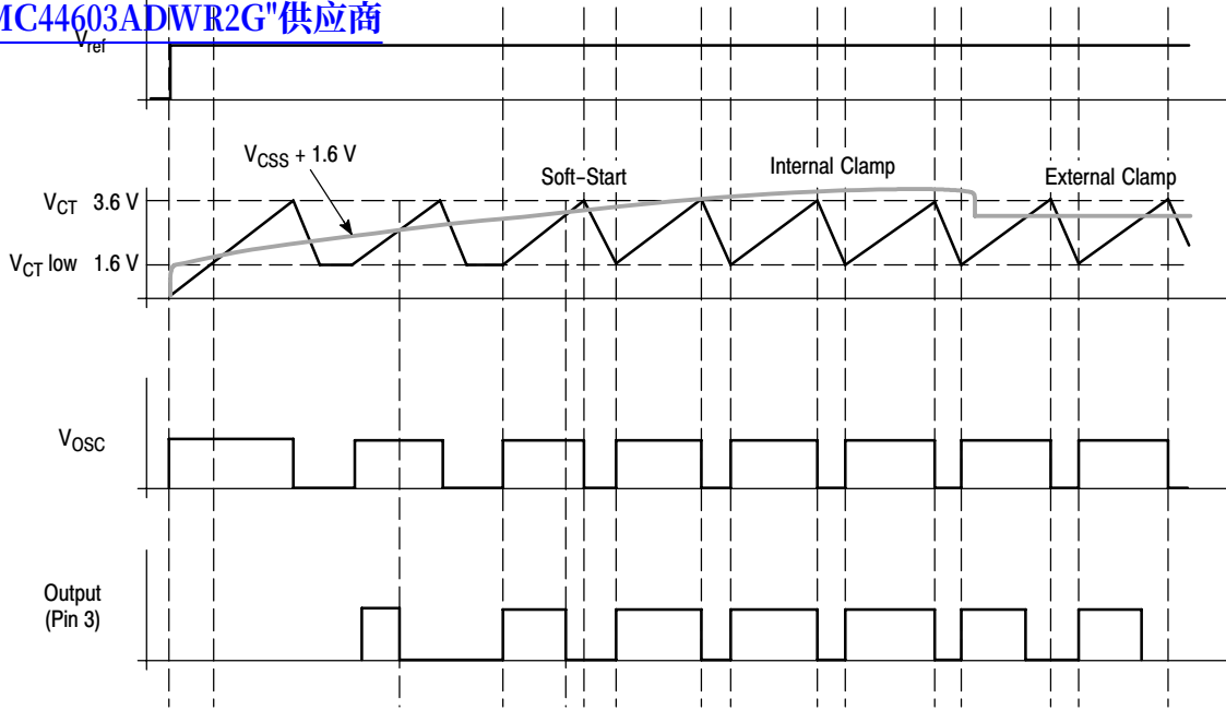
Figure 32. Soft-Start & D_{max}
