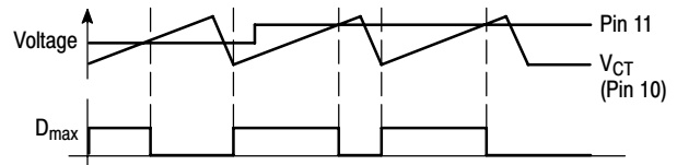
Figure 44. Maximum Duty Cycle Control
