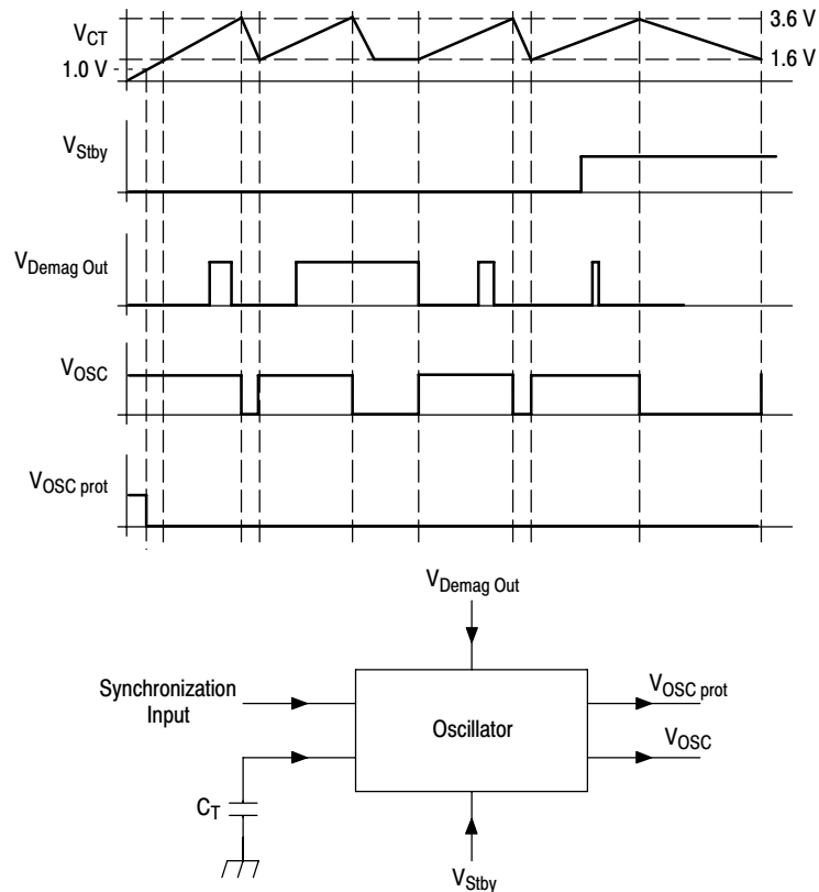
Figure 31. Oscillator
