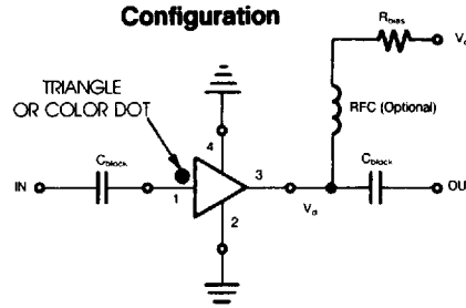
Typical Biasing Configuration
