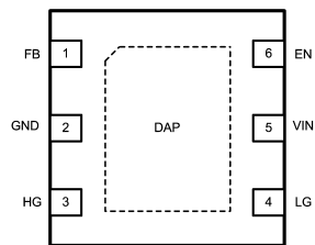
6-Lead LLP (3mm x 3mm) NS Package Number SDE06A
