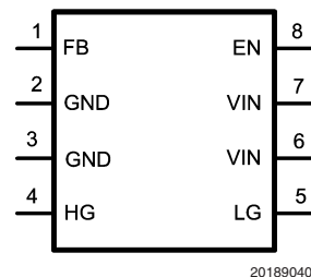
MSOP-8 NS Package Number MUA08A
