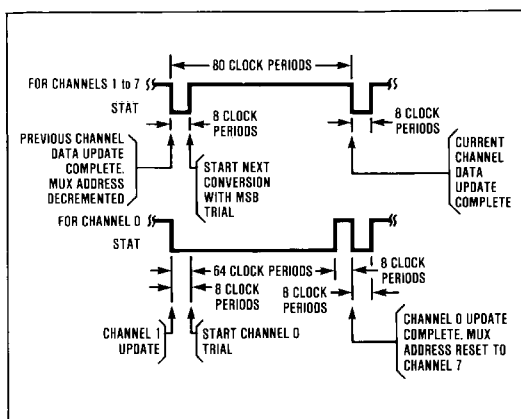
Figure 2. \overline{STAT} Timing Diagram
