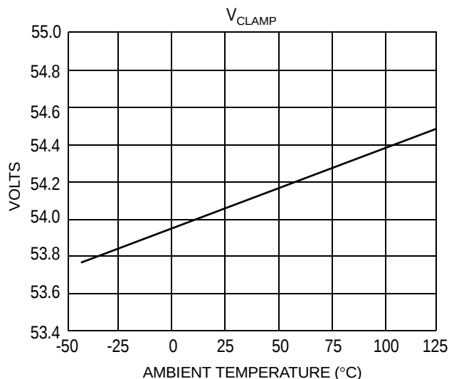
Figure 10. Output Clamp Voltage Versus Temperature
