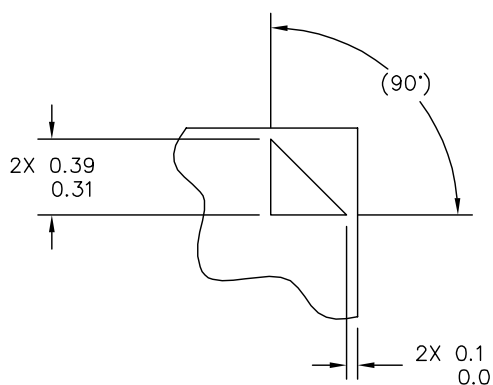
DETAIL T PREFERRED BACKSIDE PIN 1 INDEX
