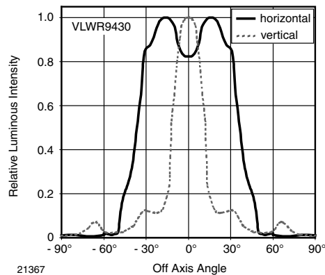
Fig. 4 - Rel. Luminous Intensity vs. Off Axis
