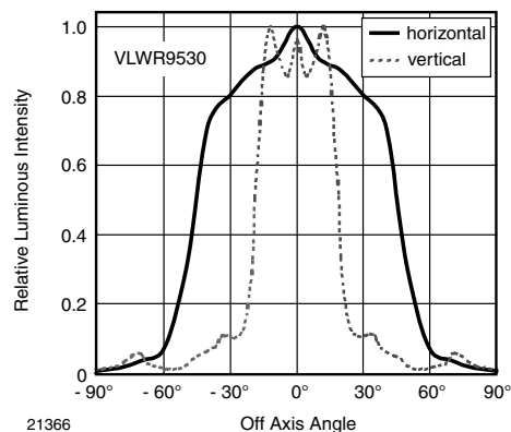
Fig. 3 - Rel. Luminous Intensity vs. Off Axis
