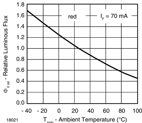
Fig. 6 - Rel. Luminous Flux vs. Ambient Temperature
