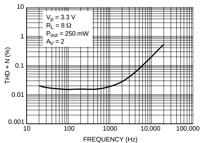
Figure 12. THD + N versus Frequency
