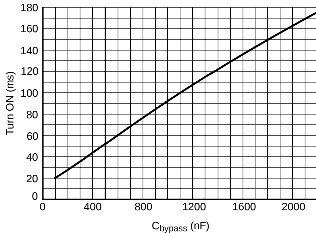
Figure 21. T_{ON} versus C_{bypass} @ V_{bat} = 3.6\text{ V} , T_A = +25^\circ\text{C}
