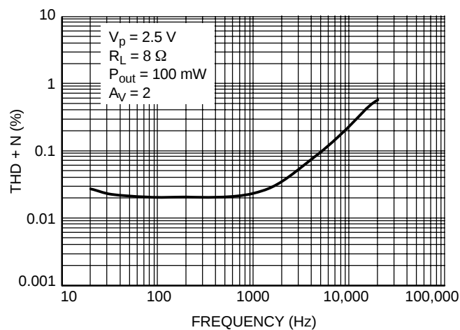
Figure 10. THD + N versus Frequency
