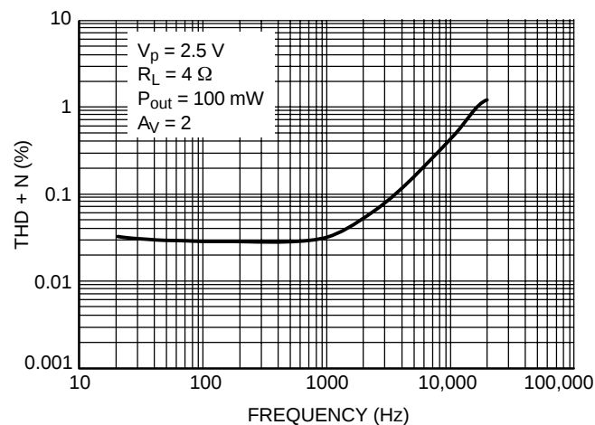
Figure 14. THD + N versus Frequency
