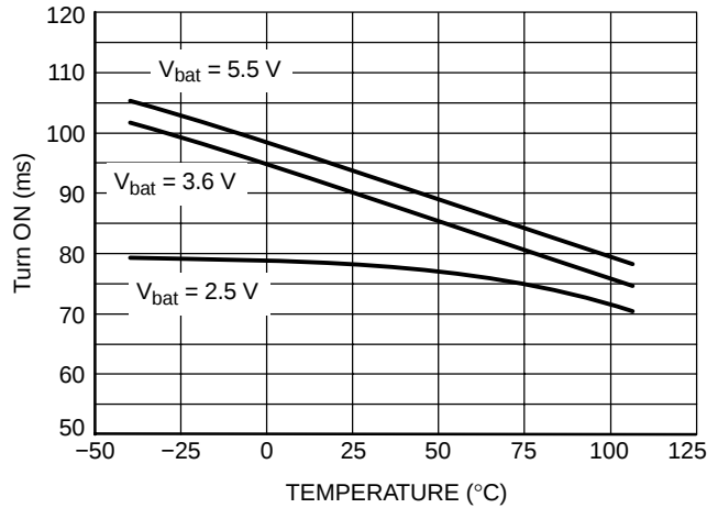
Figure 22. T_{ON} versus Temperature @ V_{bat} = 3.6\text{ V} , C_{bypass} = 1\text{ }\mu\text{F}
