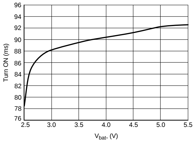
Figure 23. T_{ON} vs. V_{bat} @ C_{bypass} = 1\text{ }\mu\text{F} , T_A = +25^\circ\text{C}
