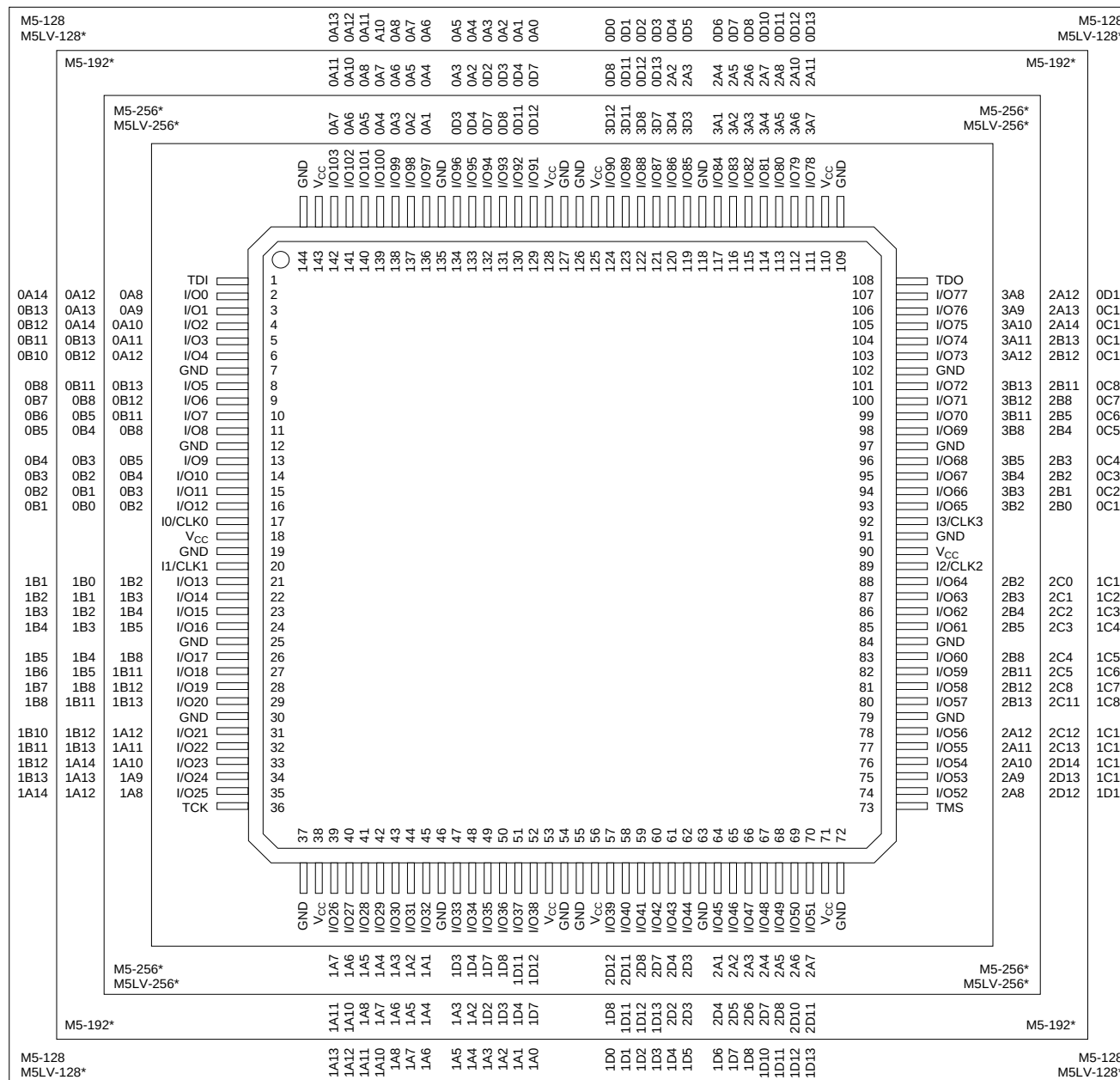
144-Pin PQFP
