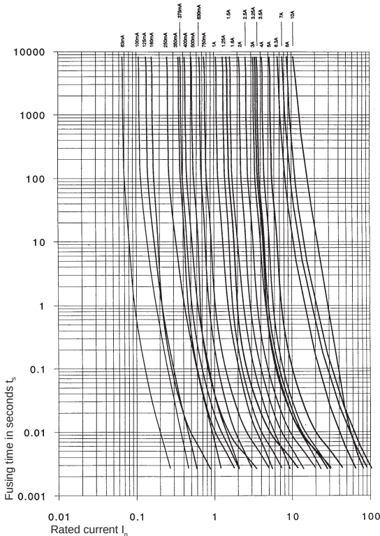
Time Current Characteristics
