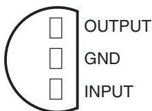
LP2950...LP (TO-226/TO-92 PACKAGE) (BOTTOM VIEW)
