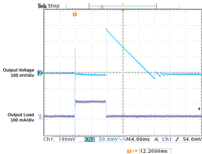
LOAD TRANSIENT RESPONSE VS TIME ( V_{OUT} = 5\text{ V} , C_L = 10\text{ }\mu\text{F} )
