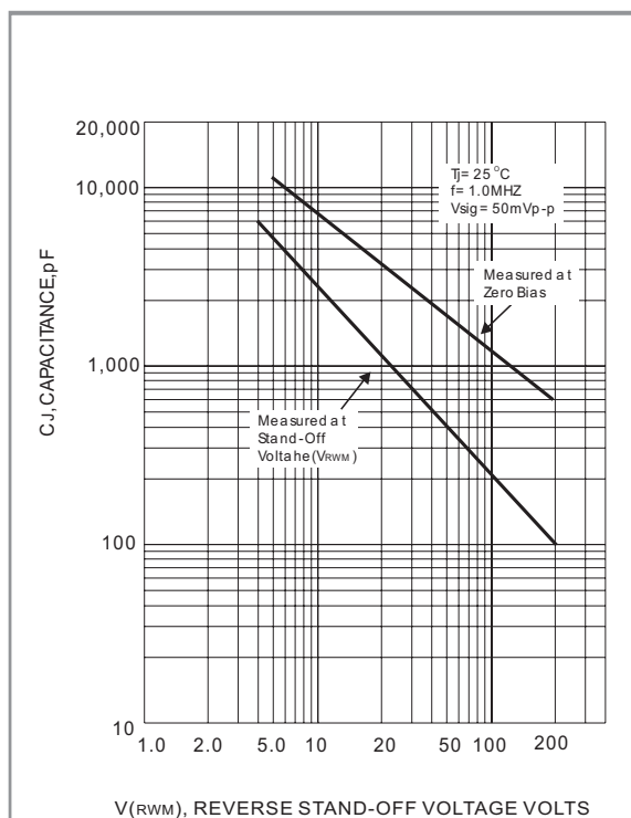
Fig.4 TYPICAL CAPACITANCE
