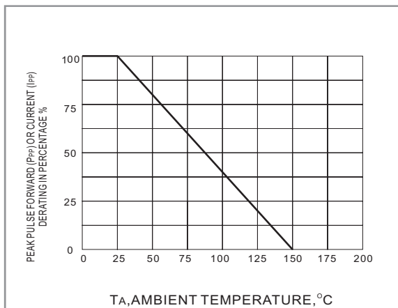
Fig.2 DERATING CURVE
