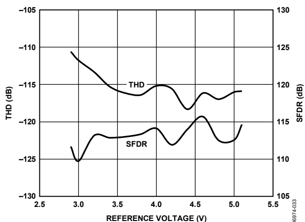
Figure 13. THD, SFDR vs. Reference Voltage
