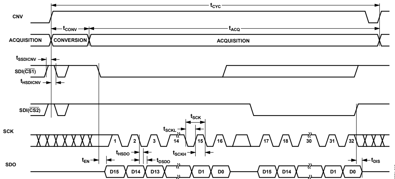
Figure 31. CS Mode, 4-Wire Without Busy Indicator Serial Interface Timing
