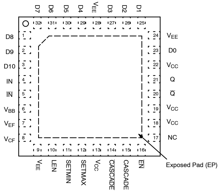
Figure 2. 32-Lead QFN Pinout (Top View)
