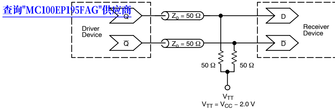
Figure 10. Typical Termination for Output Driver and Device Evaluation (See Application Note AND8020/D – Termination of ECL Logic Devices.)
