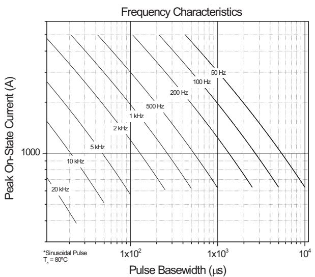
Fig. 9 - Frequency Characteristics
