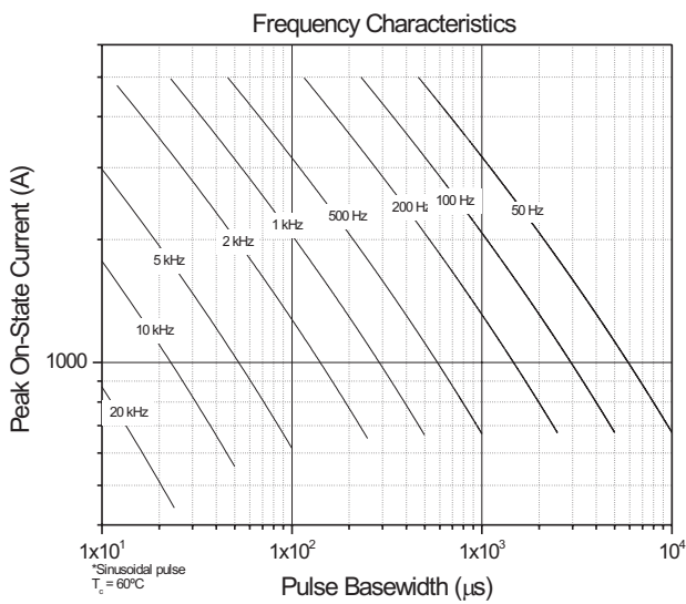
Fig. 7 - Frequency Characteristics
