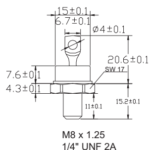
Fig. 15 - Outline Characteristics
