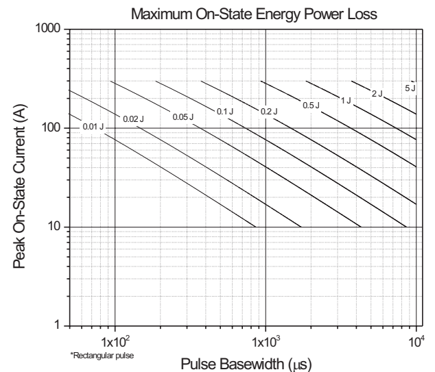
Fig. 14 - Maximum On-State Power Loss Characteristics
