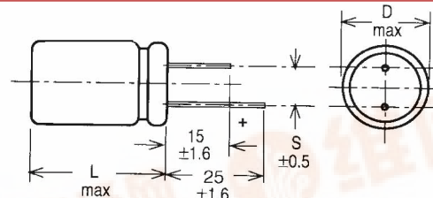
Type 361R - Two Leads
