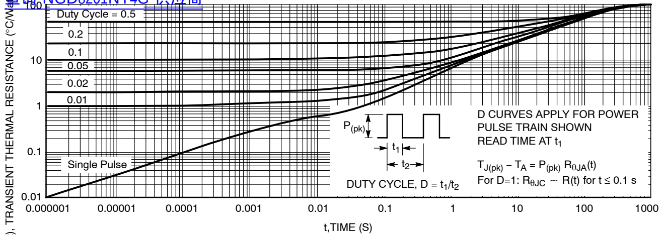
Figure 13. Minimum Pad Transient Thermal Resistance (Non-normalized Junction-to-Ambient)
