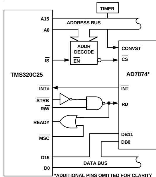
Figure 14. AD7874-TMS320C25 Interface
