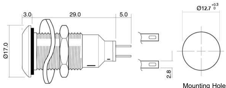
Mounting Hole
