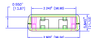
ASSEMBLED VIEW
