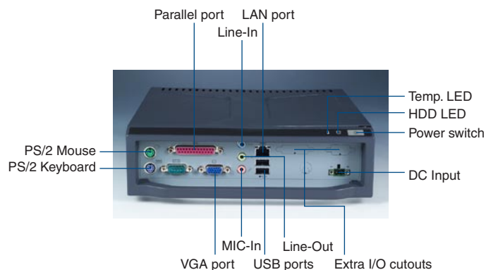
ARK-6310-3M01E/02E Front IO view
