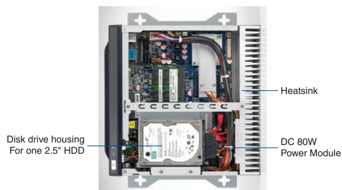
ARK-6310-6M01E Inside view
