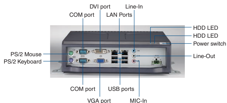
ARK-6310-6M01E Front IO view
