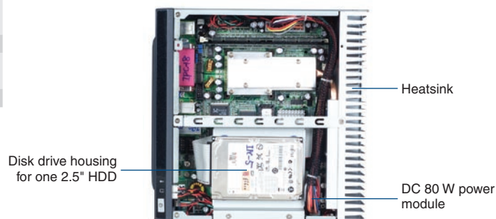
ARK-6310-3M01E/02E Inside view
