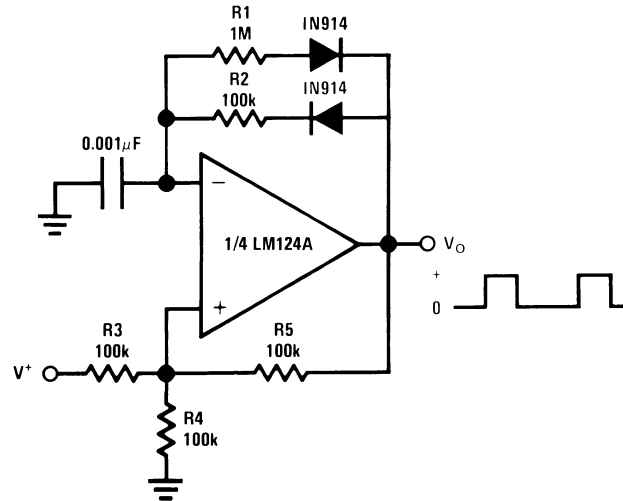
Pulse Generator
