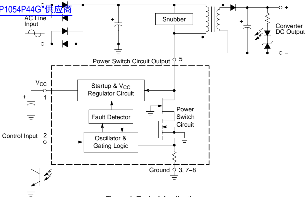
Figure 1. Typical Application
