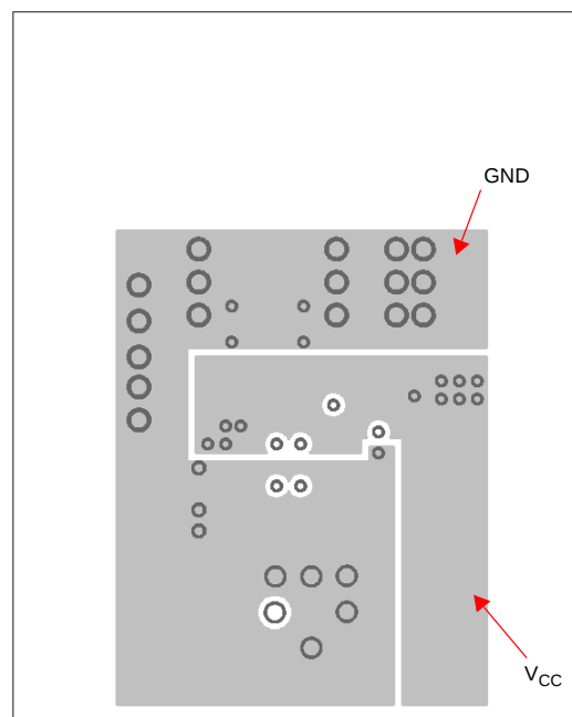
Figure 26: RF part: bottom layer
