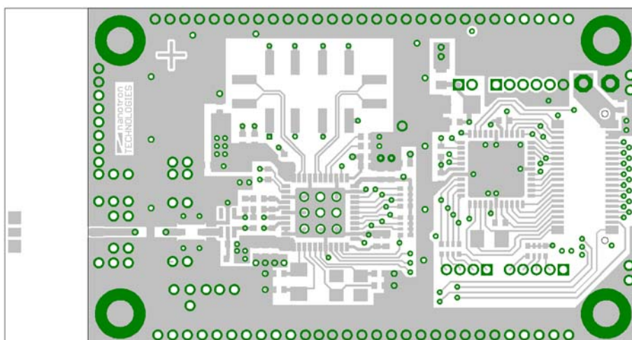
Figure 37: Reference design: top layer
