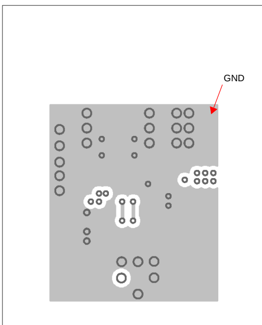
Figure 25: RF part: layer 3
