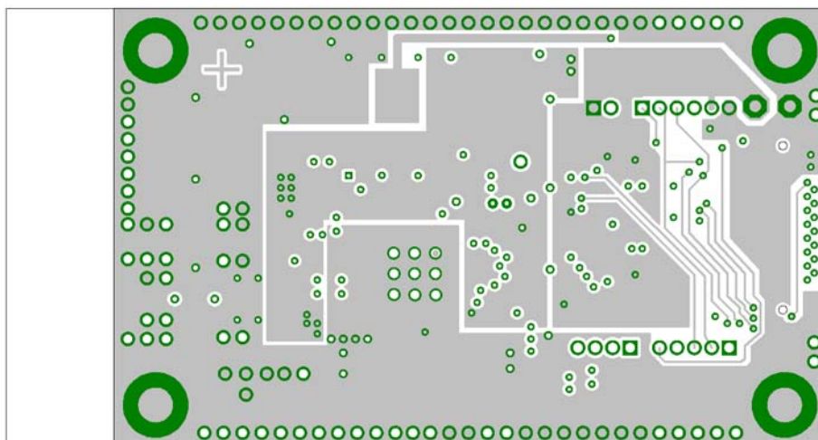
Figure 40: Reference design: bottom layer
