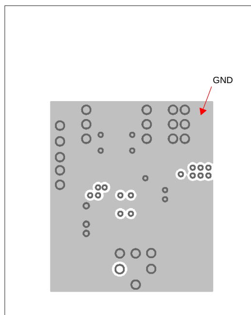
Figure 24: RF part: layer 2
