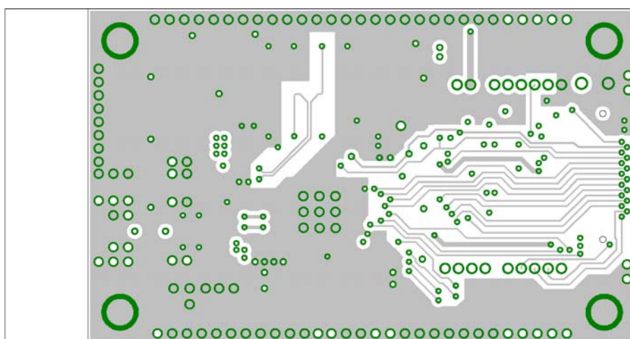
Figure 39: Reference design: layer 3
