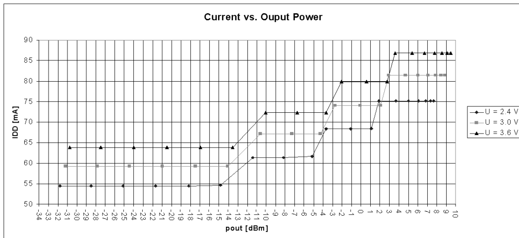
Figure 15: Total current consumption (IDD[mA] by output power [dBm])
