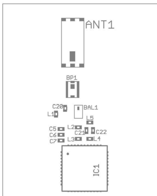
Figure 22: RF part: names
