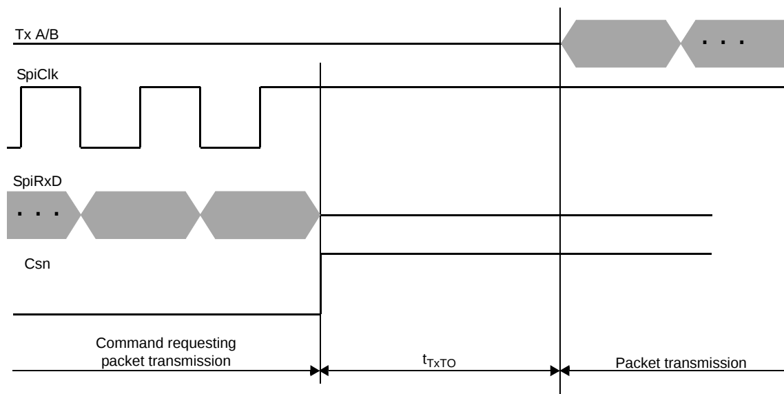
Figure 9: Turn-on time TX: time = t_{\text{TxTO}}
