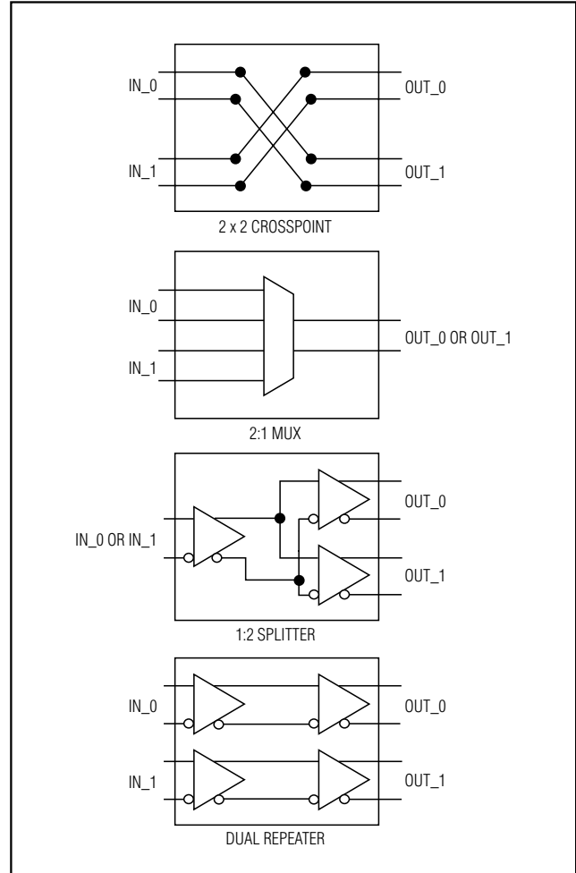
Figure 7. Programmable Configurations
