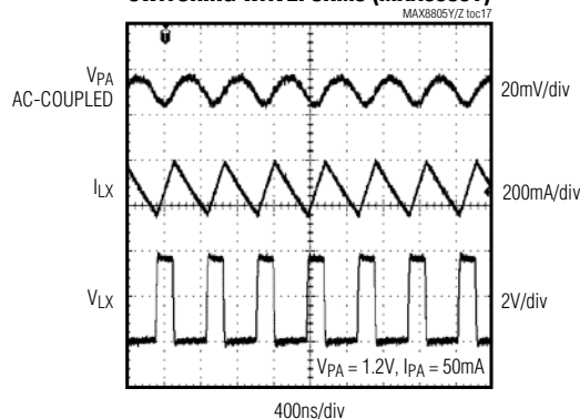
PA STEP-DOWN CONVERTER LIGHT-LOAD SWITCHING WAVEFORMS (MAX8805Y)
