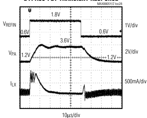
PA STEP-DOWN CONVERTER AUTOMATIC BYPASS-FET TRANSIENT RESPONSE
