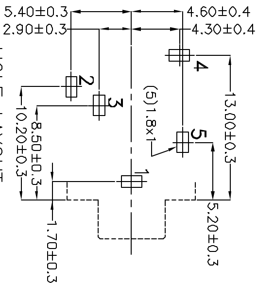
HOLE LAYOUT (TOP VIEW)
