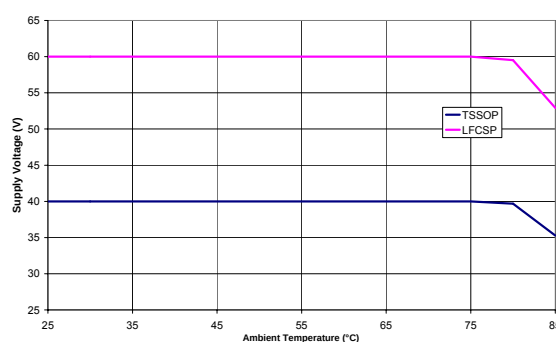
Figure 42. Maximum Supply Voltage Vs Ambient Temperature
