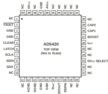
Figure 6. LFCSP Pin Configuration
