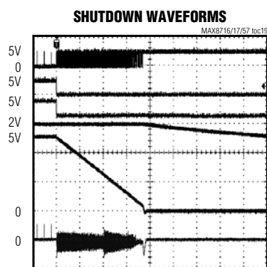
A. DL2, 10V/div B. ON2, 10V/div C. PG00D2, 10V/div D. REF, 2V/div E. OUT2, 2V/div F. I_{LX2} , 2.5A/div 1.0k \Omega LOAD ON OUT2 SKIP2 = GND
