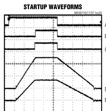
A. ON1/ON2, 5V/div B. PG00D1, 10V/div C. PG00D2, 10V/div D. OUT2, 2V/div E. OUT1, 2V/div
