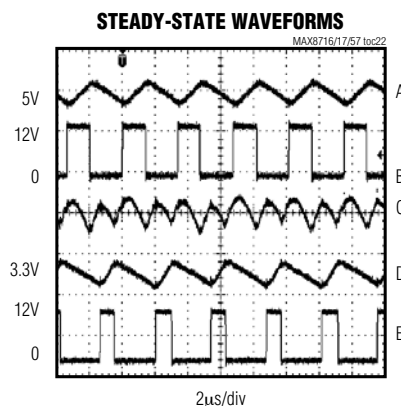
A. OUT2, 50mV/div B. LX2, 10V/div C. V_{IN} , 50mV/div D. OUT1, 50mV/div E. LX1, 10V/div 1.0A LOAD ON OUT1, 1.0A LOAD ON OUT2 SKIP1 = V_{CC} , SKIP2 = V_{CC}
