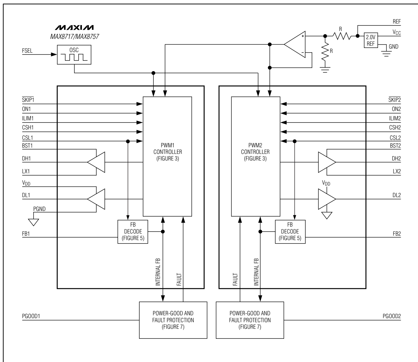
Figure 2. Functional Diagram
