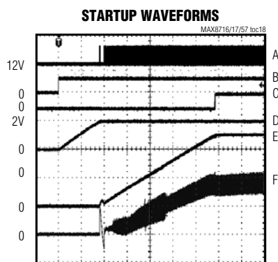
A. LX2, 20V/div B. ON2, 10V/div C. PG00D2, 10V/div D. REF, 2V/div E. OUT2, 2V/div F. I_{LX2} , 2.5A/div 1.0 \Omega LOAD ON OUT2
