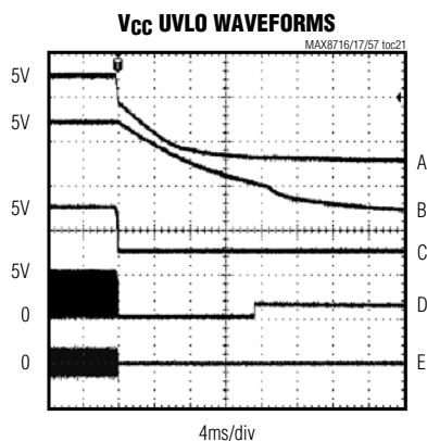
A. V_{CC} , 2V/div B. OUT2, 2V/div C. PG00D2, 5V/div D. DL2, 5V/div E. I_{LX2} , 2.5A/div 100 \Omega LOAD ON OUT2 SKIP2 = V_{CC}
