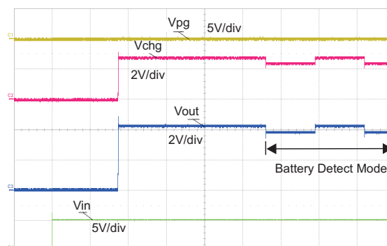
Figure 8. Hot Plug Source w/No Battery – Battery Detection
