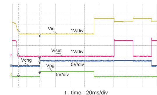
Vin swept from 5V to 3.9V to 5V, Vbat = 4V
