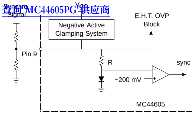
Figure 6. Synchronization
