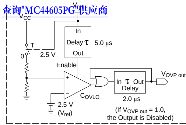
Figure 9. Overvoltage Protection
