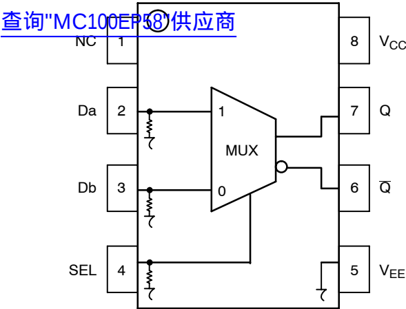
Figure 1. 8-Lead Pinout (Top View) and Logic Diagram
