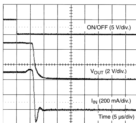
SiP4280A-3 Turn-Off ( V_{IN} = 5\text{ V} , R_{LOAD} = 10\ \Omega )
