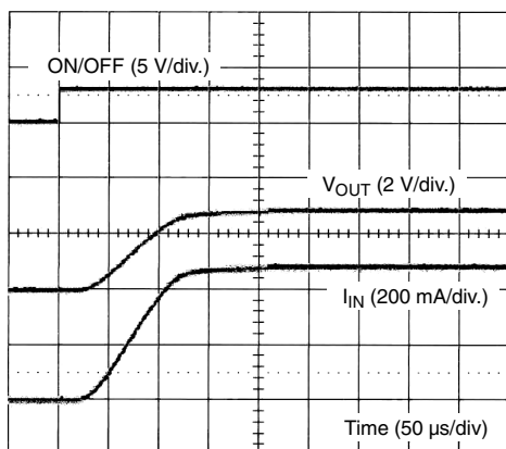
SiP4280A-3 Turn-On ( V_{IN} = 3\text{ V} , R_{LOAD} = 6\ \Omega )
