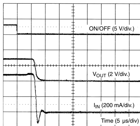
SiP4280A-3 Turn-Off ( V_{IN} = 3\text{ V} , R_{LOAD} = 6\ \Omega )
