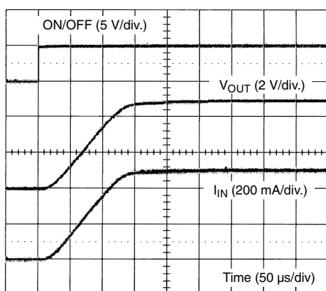
SiP4280A-3 Turn-On ( V_{IN} = 5\text{ V} , R_{LOAD} = 10\ \Omega )
