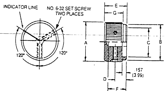
STRAIGHT KNURL WITH TOP AND SIDE INDICATOR
